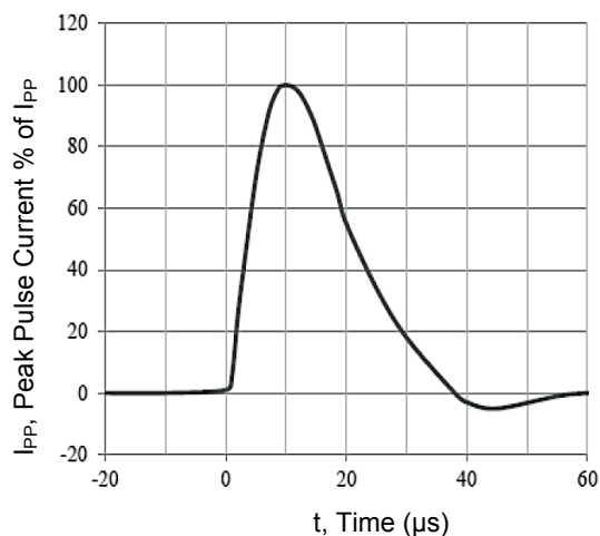
Figure 3. 8 X 20μs Pulse Waveform
