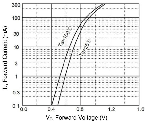
Figure 1. Forward Characteristics
