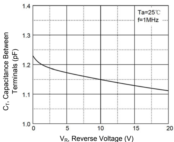
Figure 3. Capacitance Characteristics
