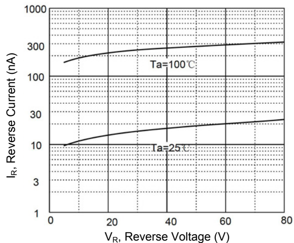
Figure 2. Reverse Characteristics
