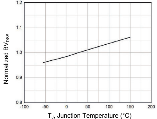
Figure 4. Normalized BV_{DSS} vs. Junction Temperature
