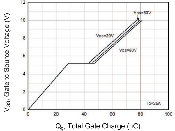
Figure 8. Gate Charge
