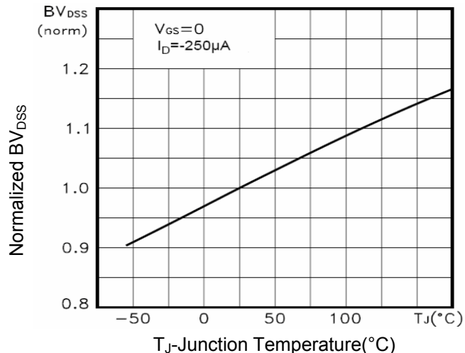
Fig.21 BV_{DS} vs Junction Temperature
