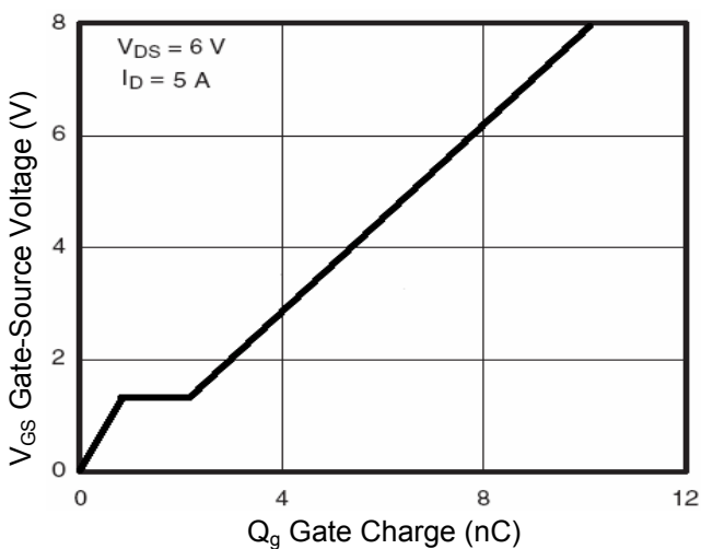
Fig.9 Gate Charge
