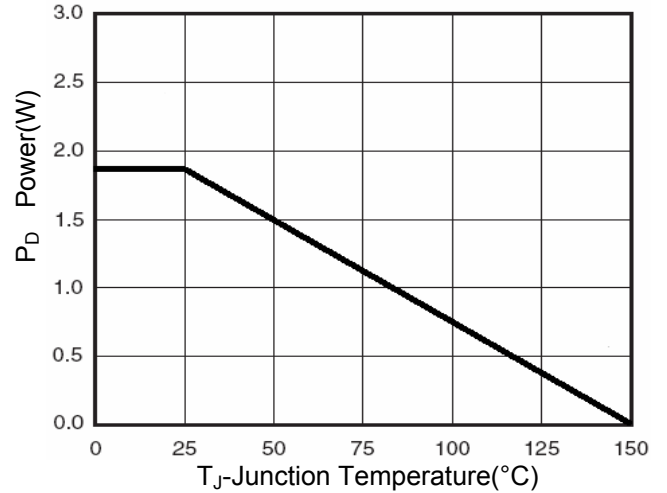
Fig.8 Power Dissipation
