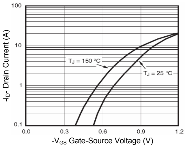
Fig.16 Transfer Characteristics
