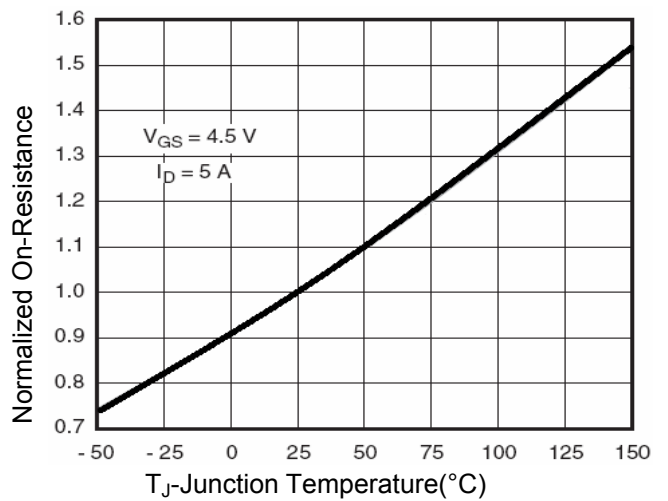
Fig.6 Drain-Source On-Resistance
