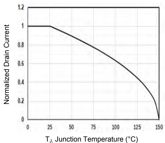
Figure 6. Normalized Drain Current vs. Junction Temperature
