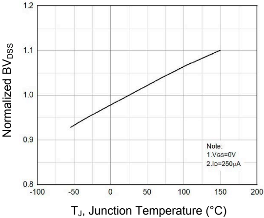
Figure 5. Normalized BV_{DS} vs. Junction Temperature
