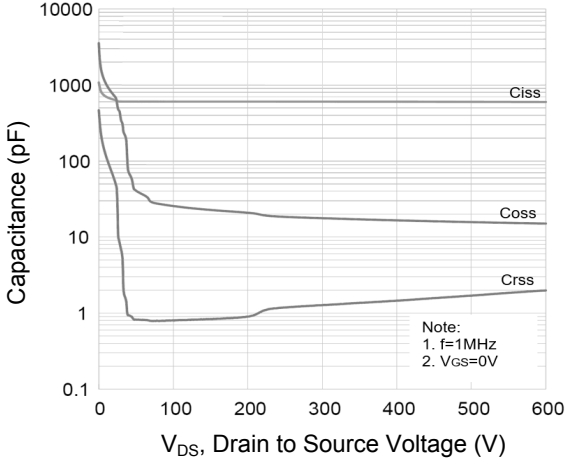
Figure 7. Capacitance Characteristic
