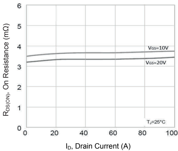
Figure 5. Drain to Source On-Resistance vs. I_D
