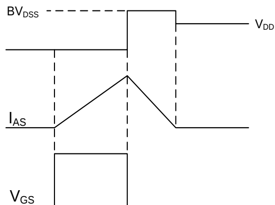
Fig.8 EAS Waveform
