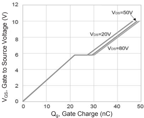
Figure 3. Gate Charge
