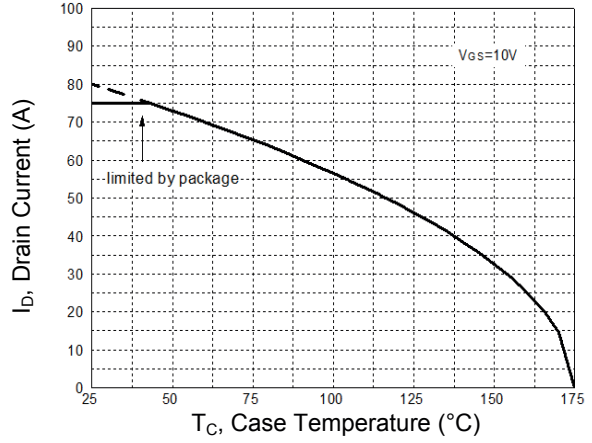
Figure 2. Drain Current vs. Case Temperature
