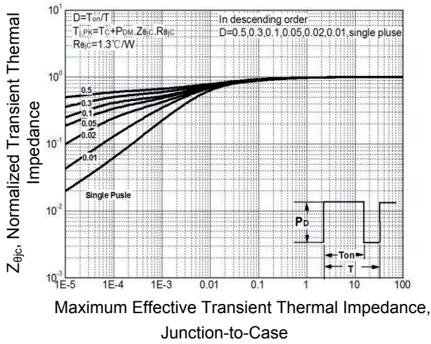
Figure 9. Max. Thermal Transient Impedance
