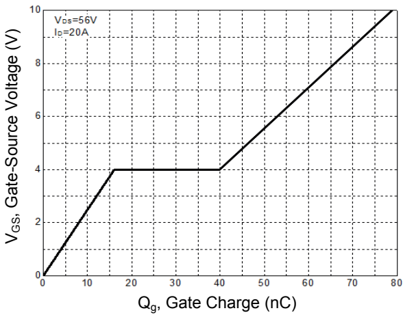
Figure 3. Gate Charge.
