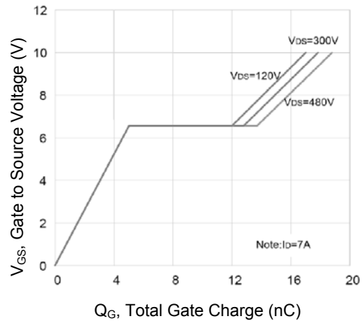
Figure 6. Gate Charge
