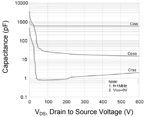
Figure 7. Capacitance Characteristics
