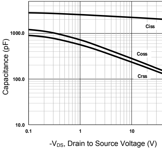
Figure 7. Capacitance Characteristics
