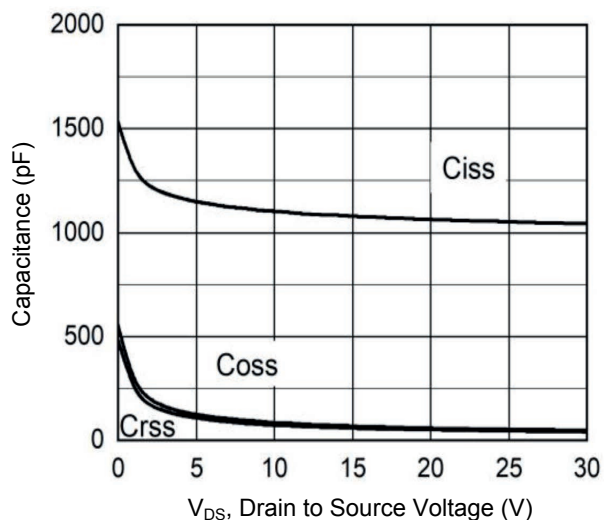
Figure 5. Capacitance Characteristics
