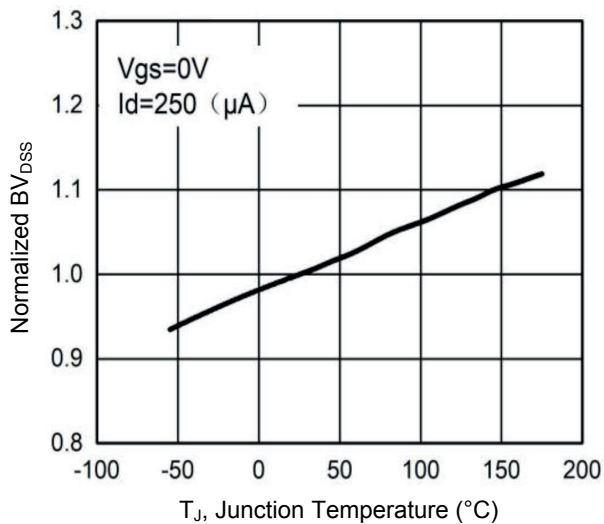
Figure 3. Normalized BV_{DS} vs. T_J
